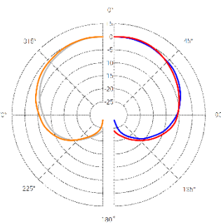
Polar Pattern
